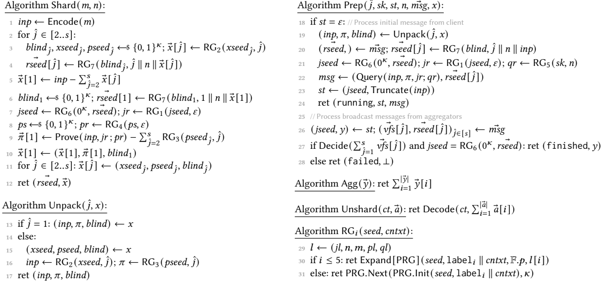
Figure 4: Definition of 1-round, s -party VDAF Prio3[FLP, PRG]. Let label_1, \dots, label_s be arbitrary, distinct bitstrings.
